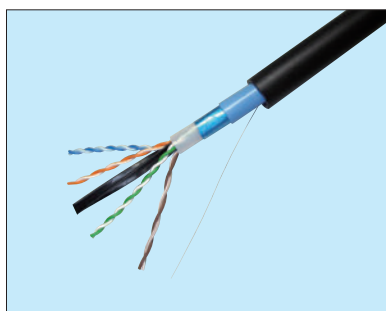
TPCC 6A - LAP 23AWG x 4P
